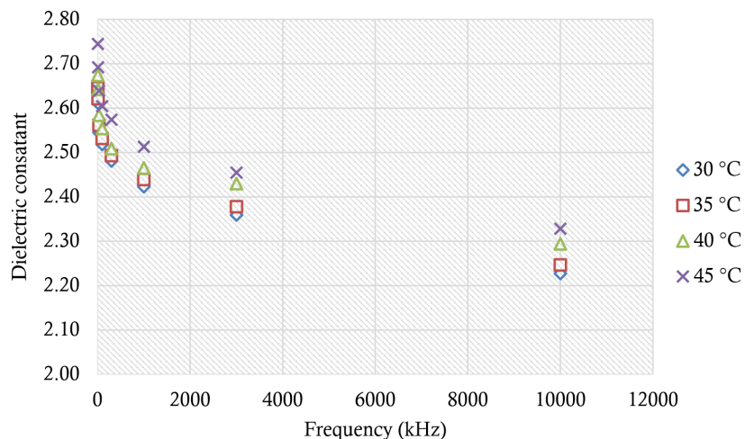
Fig. 1. Dielectric constant of barley seed at moisture content 4.1% and bulk density 0.649 g/cm 3
