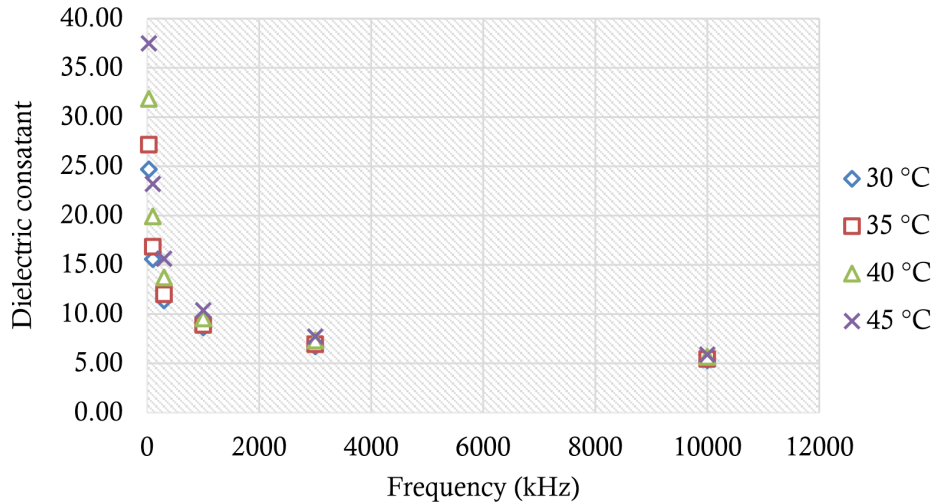
Fig. 3. Dielectric constant of barley seed at moisture content 20.1% and bulk density 0.612 g/cm 3
