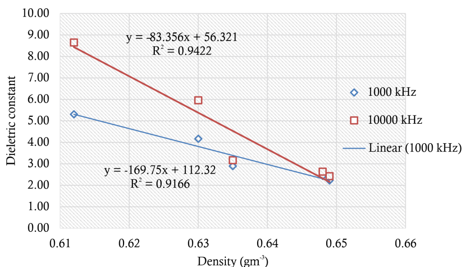
Fig. 4. Variation of dielectric constant of with barley seed density at different frequencies
