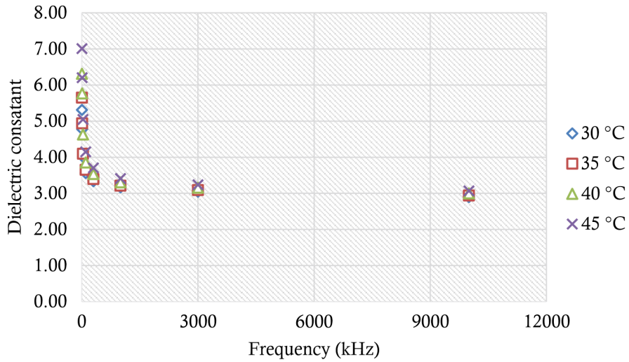
Fig. 2. Dielectric constant of barley seed at moisture content 11.0% and bulk density 0.630 g/cm 3
